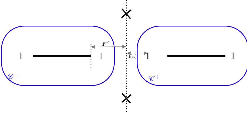
Figure 6.3: Cartoon depicting an approximation of \sigma(\mathcal{H}(u)) for u \in \text{Adm}(\Lambda) (on the real axis) and the contours \mathcal{C}^- and \mathcal{C}^+ . The positive constants \mathbf{d}(u) and \mathbf{d}^{\text{ref}} are also displayed.
