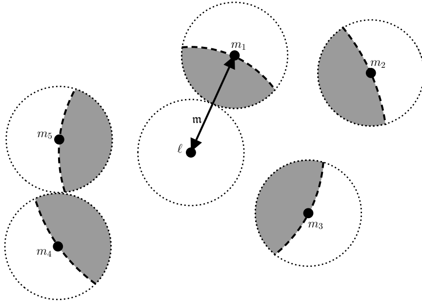
Figure B.1: Schematic plot to demonstrate the proof of Lemma B.1. Dotted circles represent the pairwise disjoint sets B_{\mathfrak{m}/2}(\mathbf{r}_m) . Dashed arcs lie on \partial B_{r_{\ell m}}(\mathbf{r}_\ell) . For \mathbf{r} in the shaded region nearest m_j (i.e. \mathbf{r} \in B_{\mathfrak{m}/2}(\mathbf{r}_{m_j}) \cap B_{r_{\ell m_j}}(\mathbf{r}_\ell) ), we have e^{-\gamma r_{\ell m_j}} \leq e^{-\gamma |\mathbf{r} - \mathbf{r}_\ell|} . Moreover, the volume of each shaded region is bounded below by c_d \mathfrak{m}^d = \mathcal{L}_d(B_{\mathfrak{m}/2}(\mathbf{r}_{m_1}) \cap B_{r_{\ell m_1}}(\mathbf{r}_\ell)) since r_{\ell m_1} = \mathfrak{m} .
