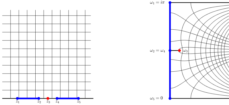
Figure 4.3: The Schwarz–Christoffel mapping G_E with E = [z_1, z_2] \cup [z_4, z_5] which maps the upper half plane (left) onto the infinite slit strip \{\omega \in \mathbb{C} : \operatorname{Re} \omega > 0, \operatorname{Im} \omega \in (0, \pi)\} (right), is continuous on \{z \in \mathbb{C} : \operatorname{Re} z \geq 0\} and maps the intervals [z_1, z_2] , [z_4, z_5] to [\omega_1, \omega_2] , [\omega_4, \omega_5] \subseteq i[0, \pi] , respectively. We also plot the image of an 10 \times 10 equi-spaced grid. A parameter problem is solved in order to obtain z_3 and thus \omega_3 and \omega_2 = \omega_4 whereas the other constants are fixed. Here, we take z_1 = -1, z_2 = -\varepsilon, z_4 = \varepsilon, z_5 = 1, \omega_1 = i\pi, \omega_5 = 0 with \varepsilon = 0.3 .
